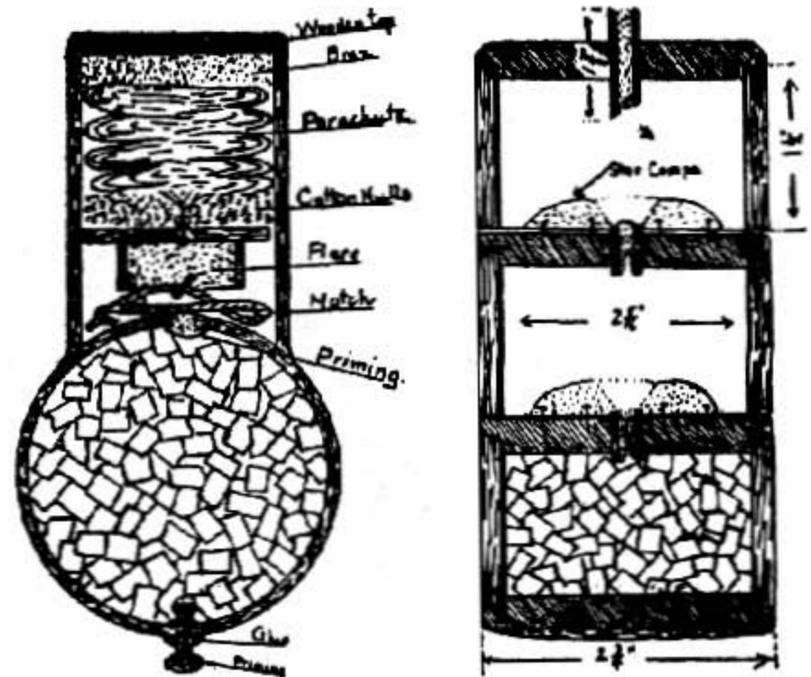
Parachute Shell. Fig. 64
